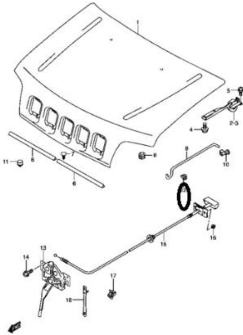
BN413V-5 E22_150 FRONT HOOD PANEL (1)
