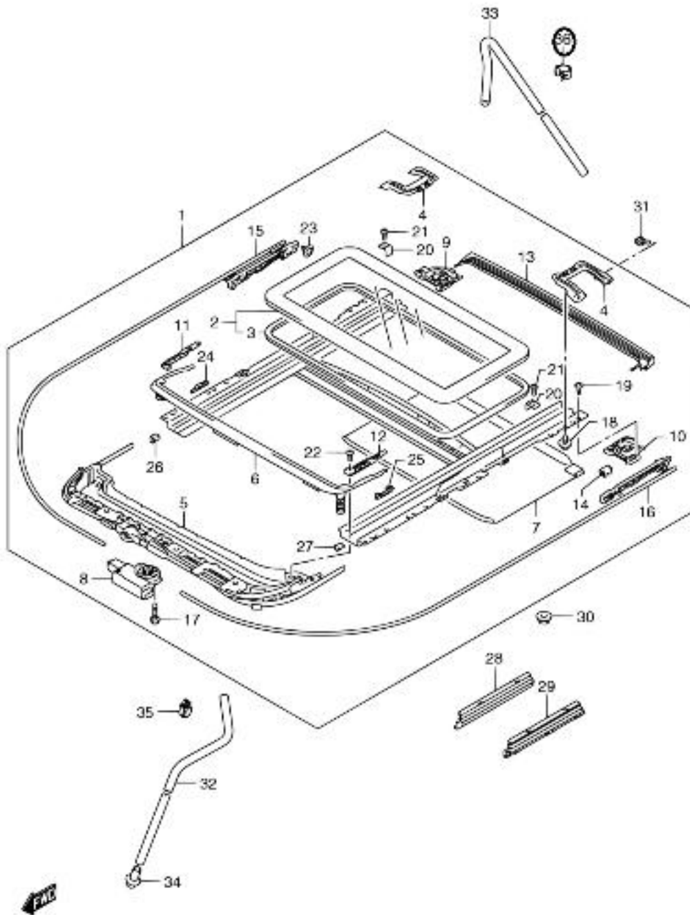
JB120W-1 E22_219 SLIDING ROOF (SUN ROOF)
