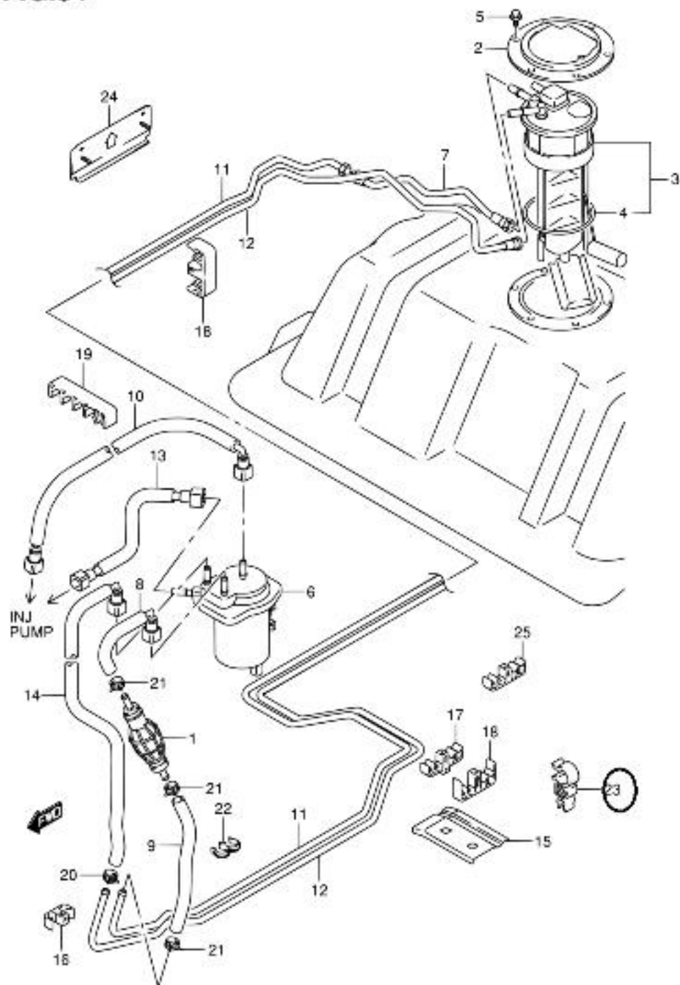
SN413V-5 E22 034 FUEL PUMP (SN415VD:1)
