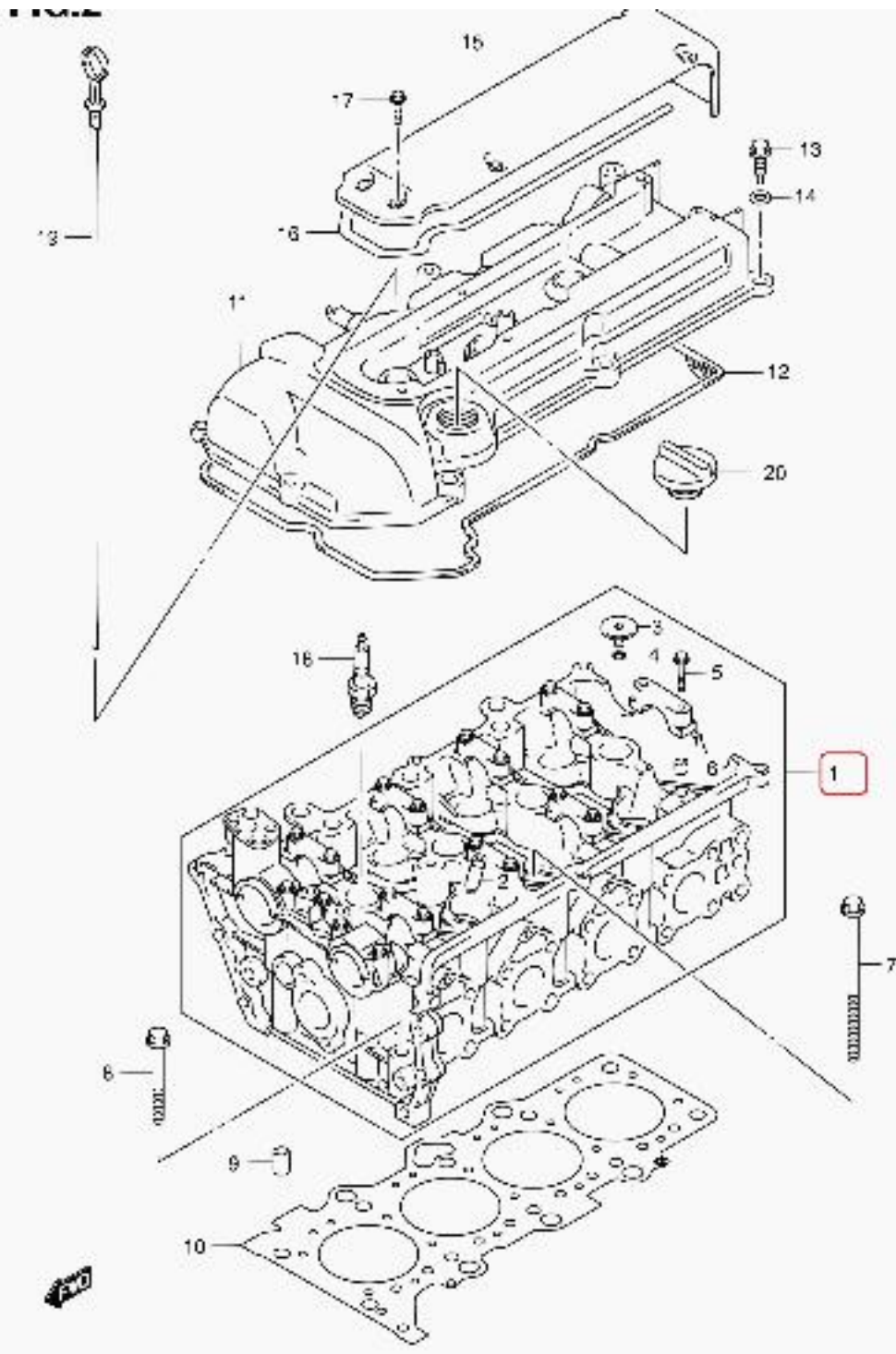
JB416X-2 E50 002 CYLINDER HEAD
