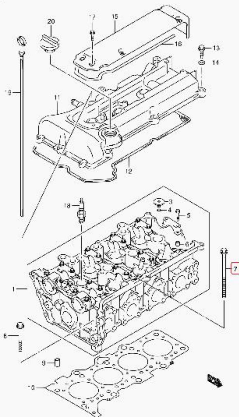
RS415 E24 003 CYLINDER HEAD (")
