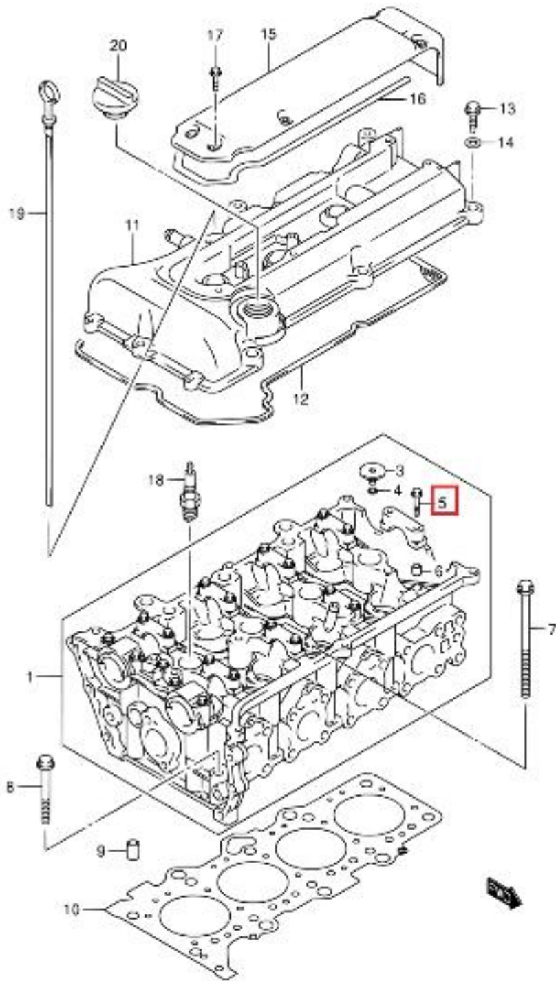
RW420 E24 007 CYLINDER HEAD (2)
