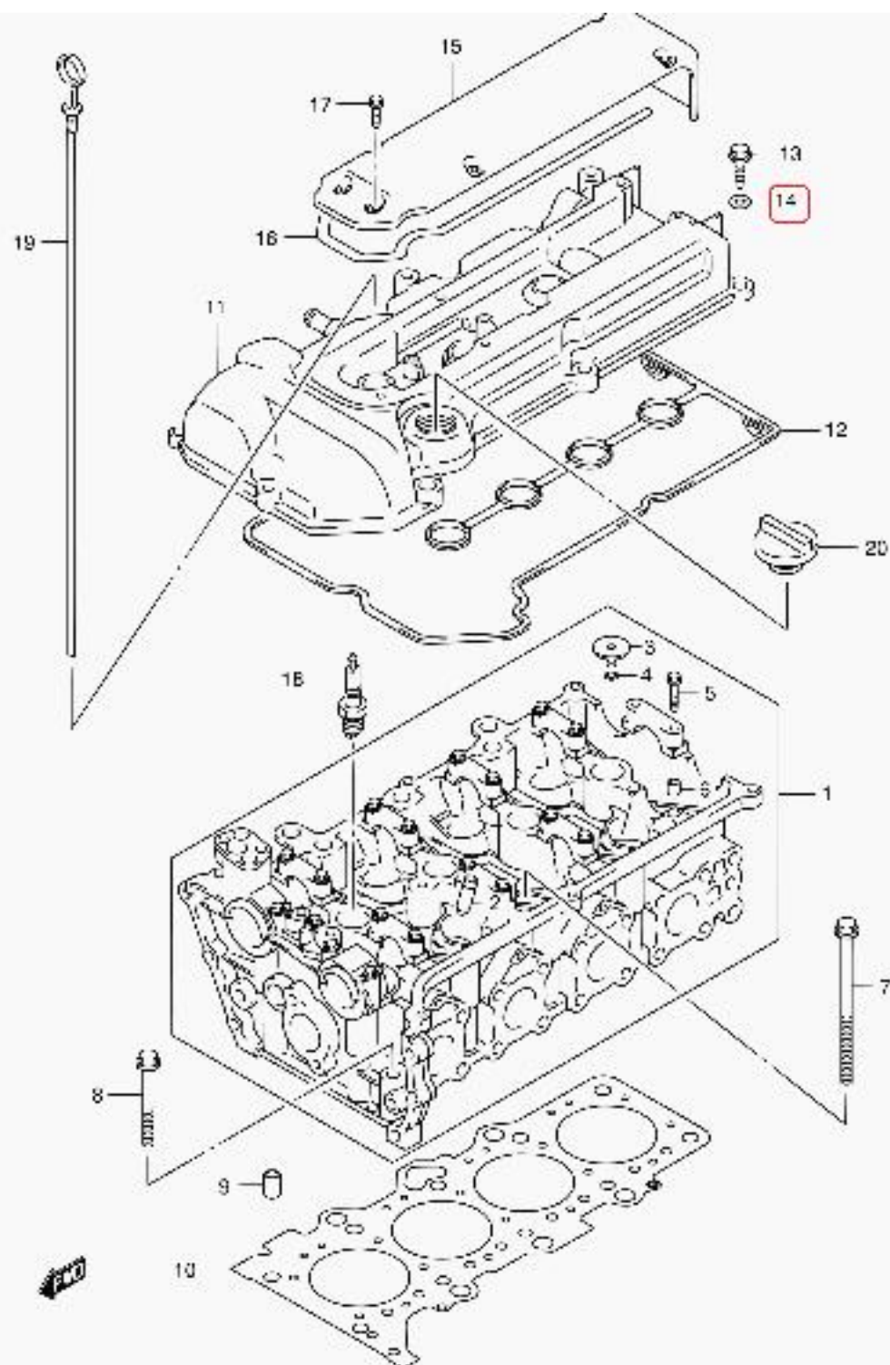
SN413V 6 F50_002 CYLINDER HEAD
