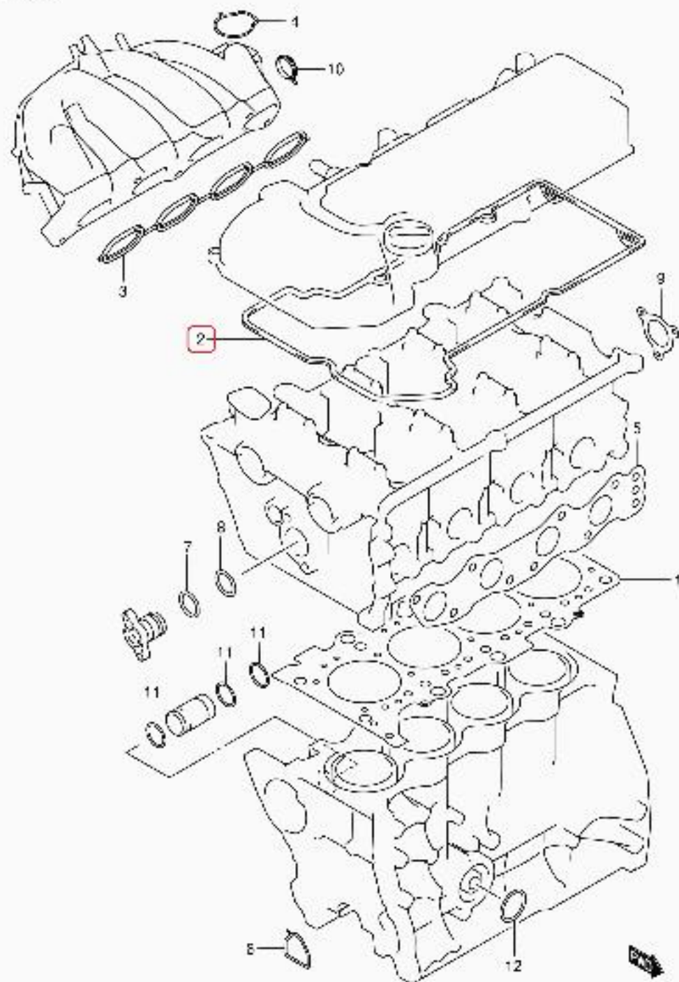
RS413 E22 001 ENGINE GASKET SET (RS413)
