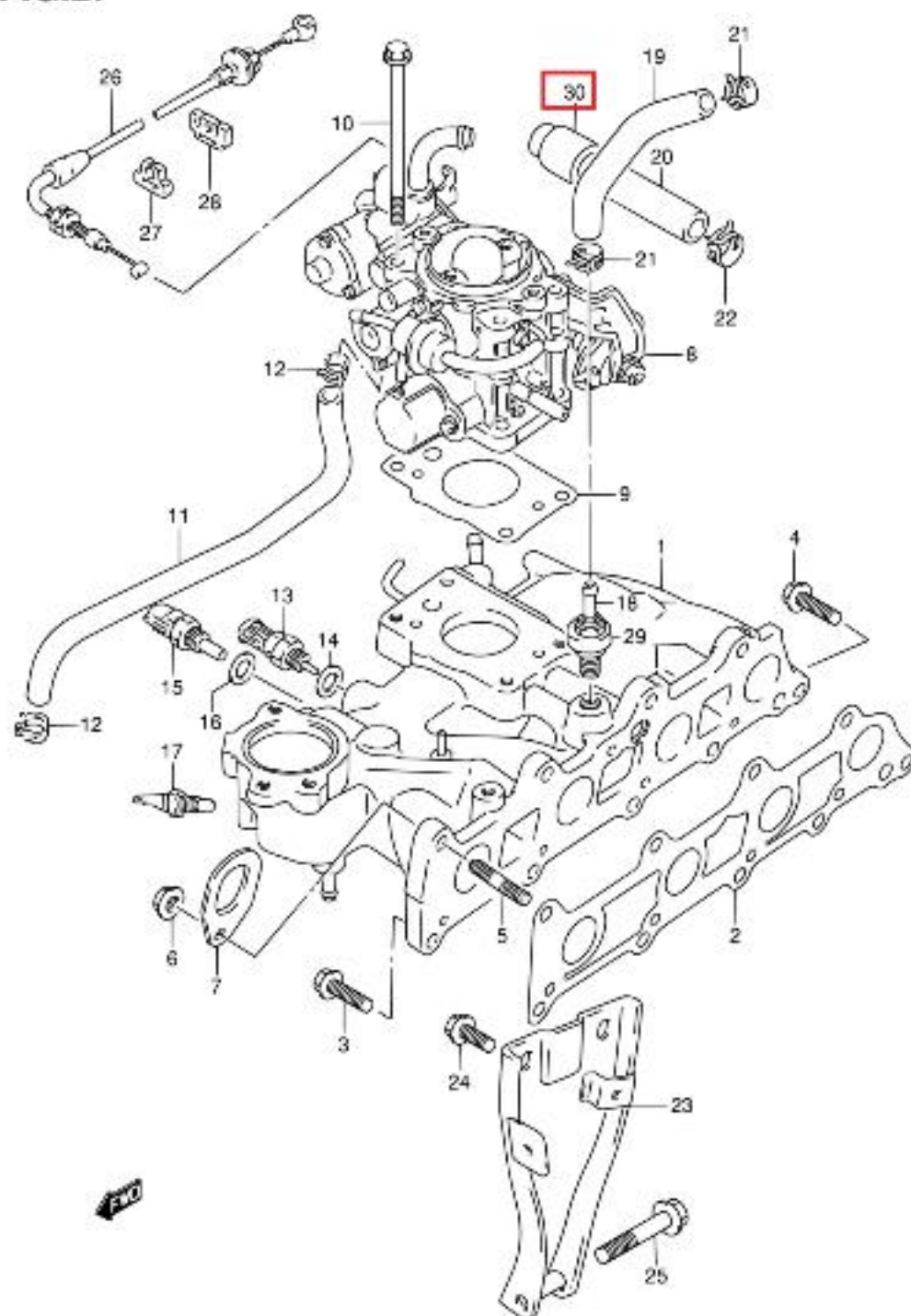
SE416 3DR E01 027 INTAKE MANIFOLD/THROTTLE BODY (8)
