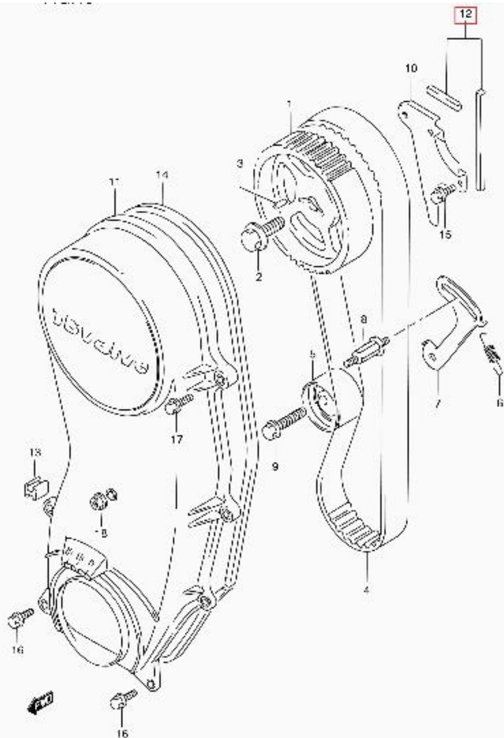
SQ416L/420L E30_016 TIMING BELT:SQ416L
