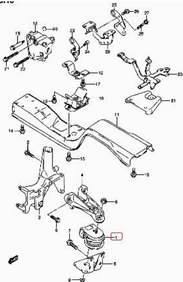
SQ420W-2 E22 019 ENGINE MOUNTING (420WD RH-2)
