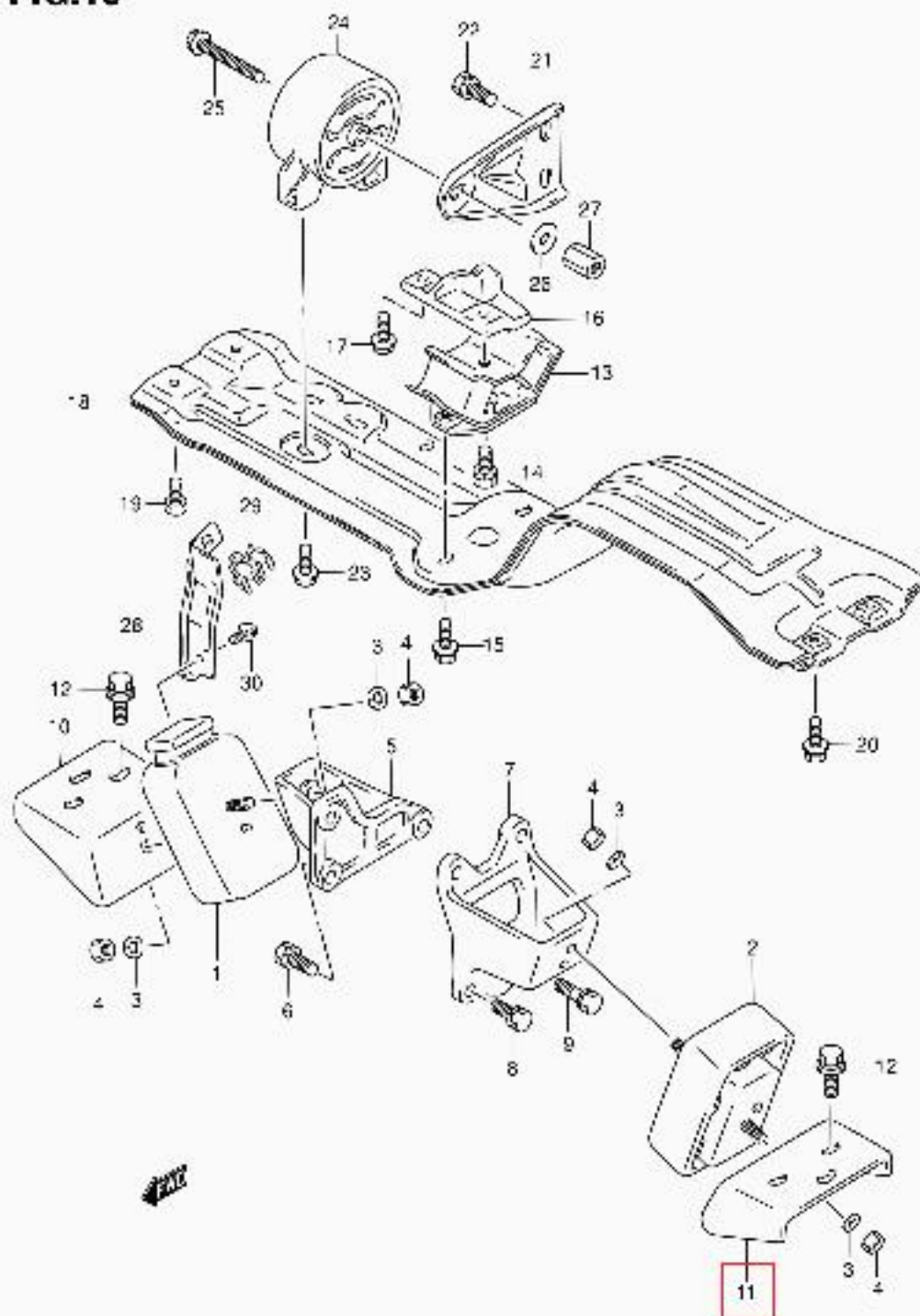
SE416 3DR E01 010 ENGINE MOUNTING (3)
