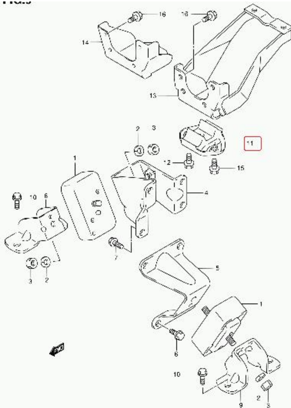
SN413V-2 E22 003 ENGINE MOUNTING (SN413V)
