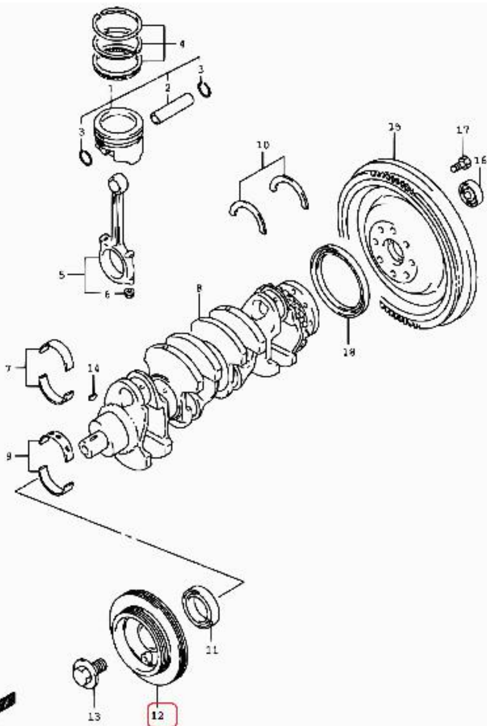
SQ430Q-2 E22_014 CRANKSHAFT (420)
