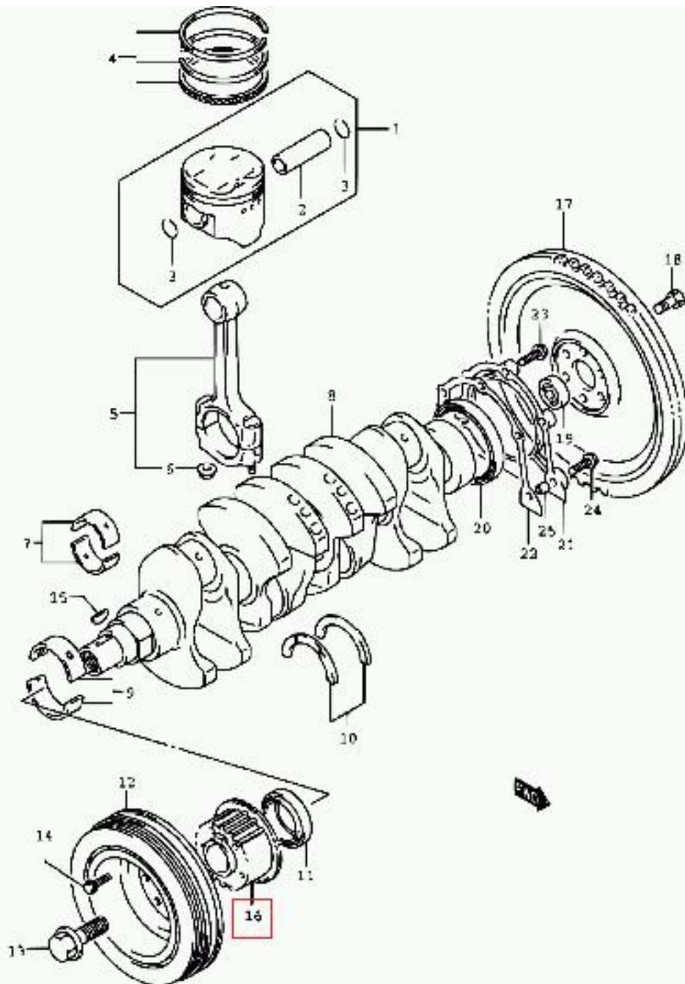
RB413 E66_007 CRANKSHAFT
