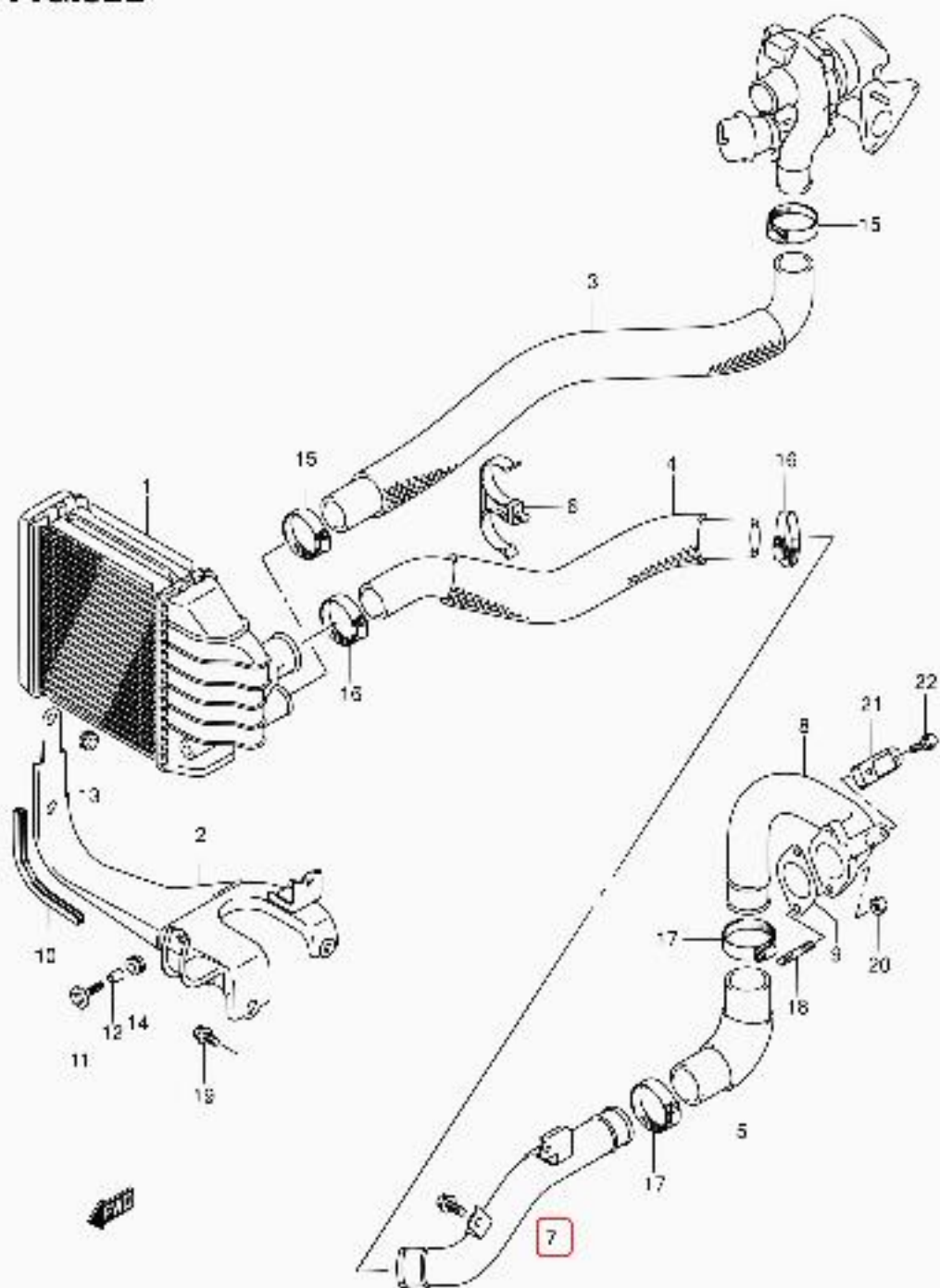
SN413V-6 E22 032B INTER COOLER (SN415VD)
