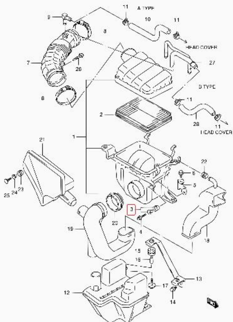
SY413-3 E01_037 AIR CLEANER SY413,SY416
