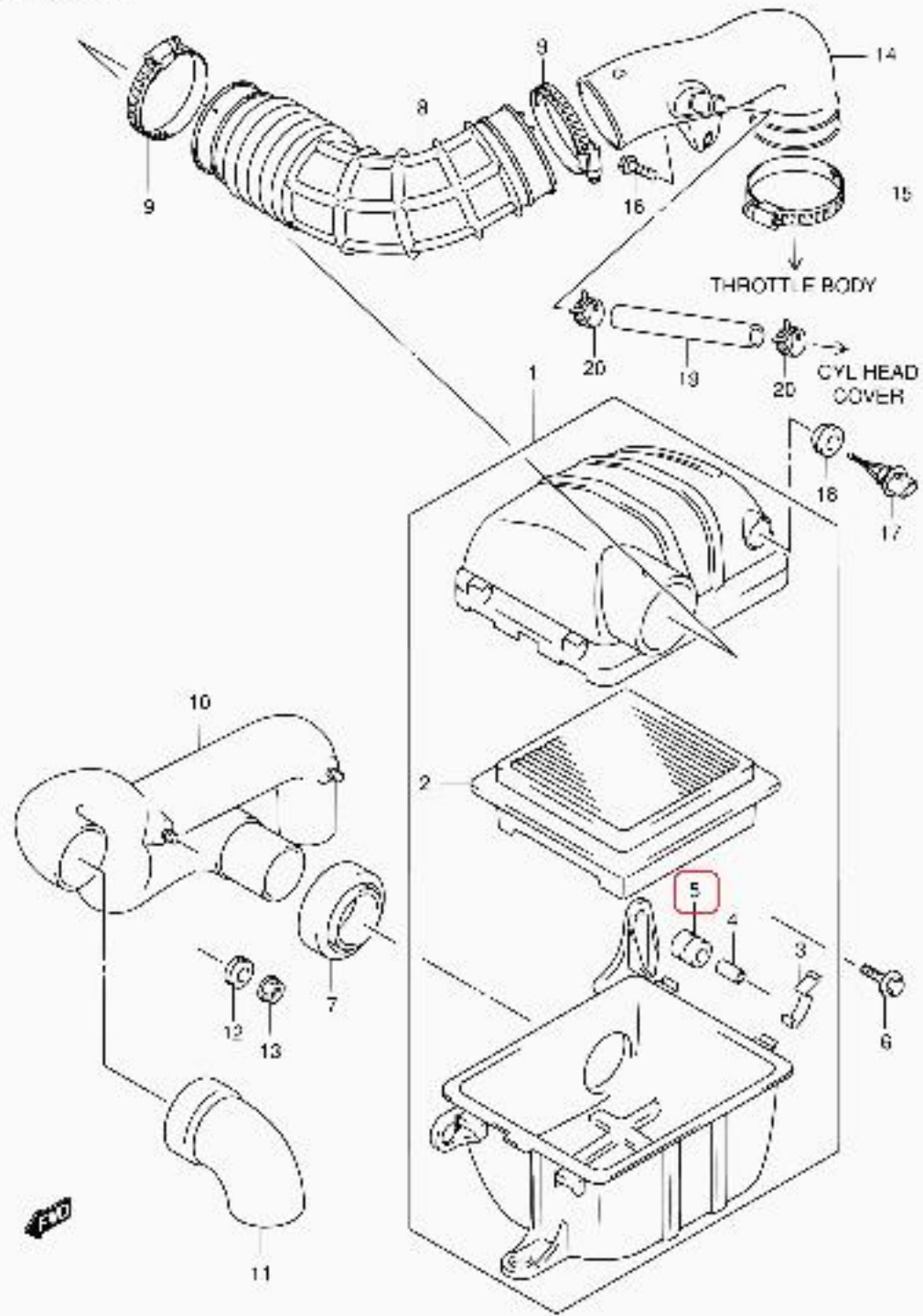
SM413V-2 E22 018 AIR CLEANER (SM413V)
