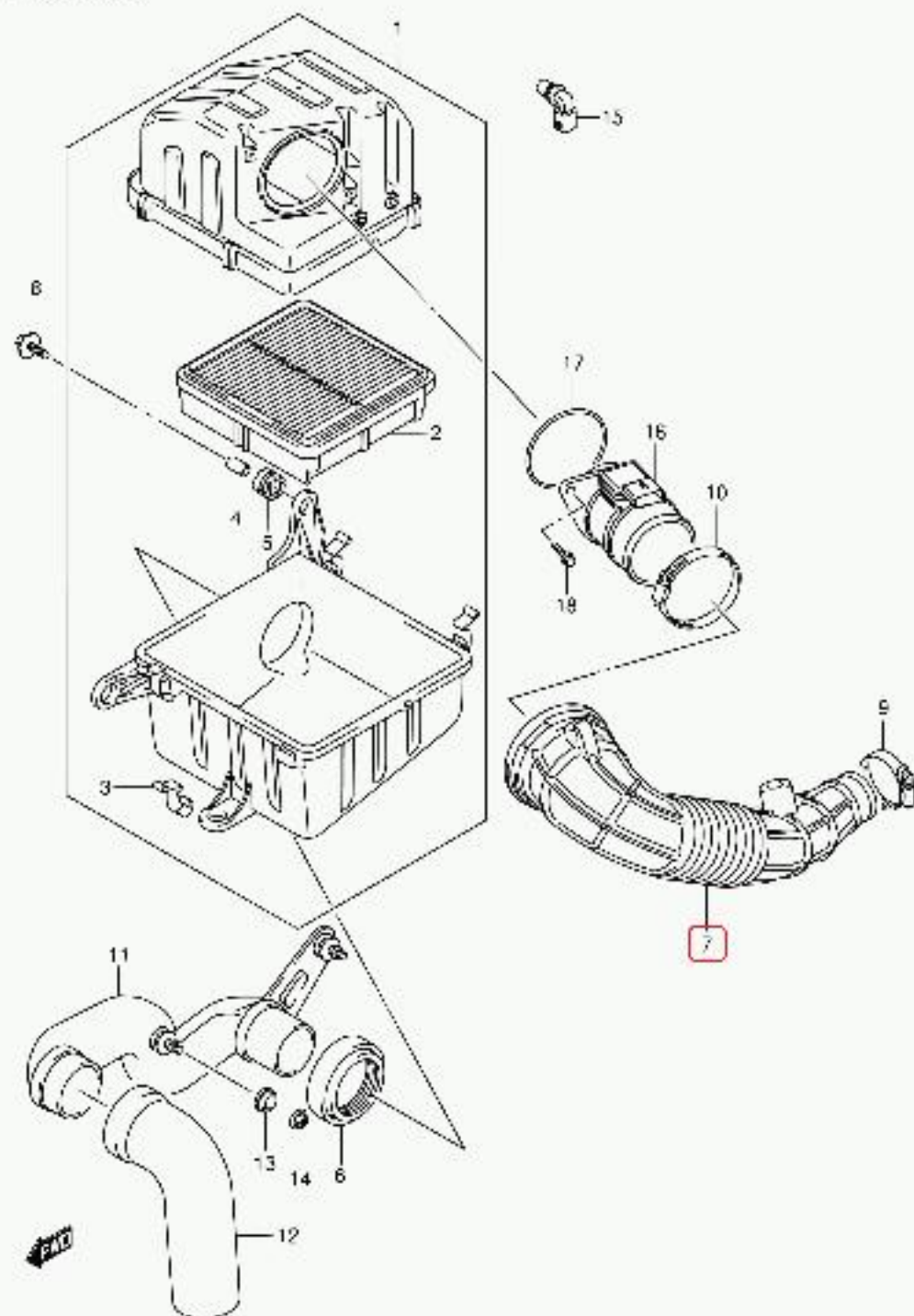
SM413V-5 E22 025A AIR CLEANER (SM415VD-2)
