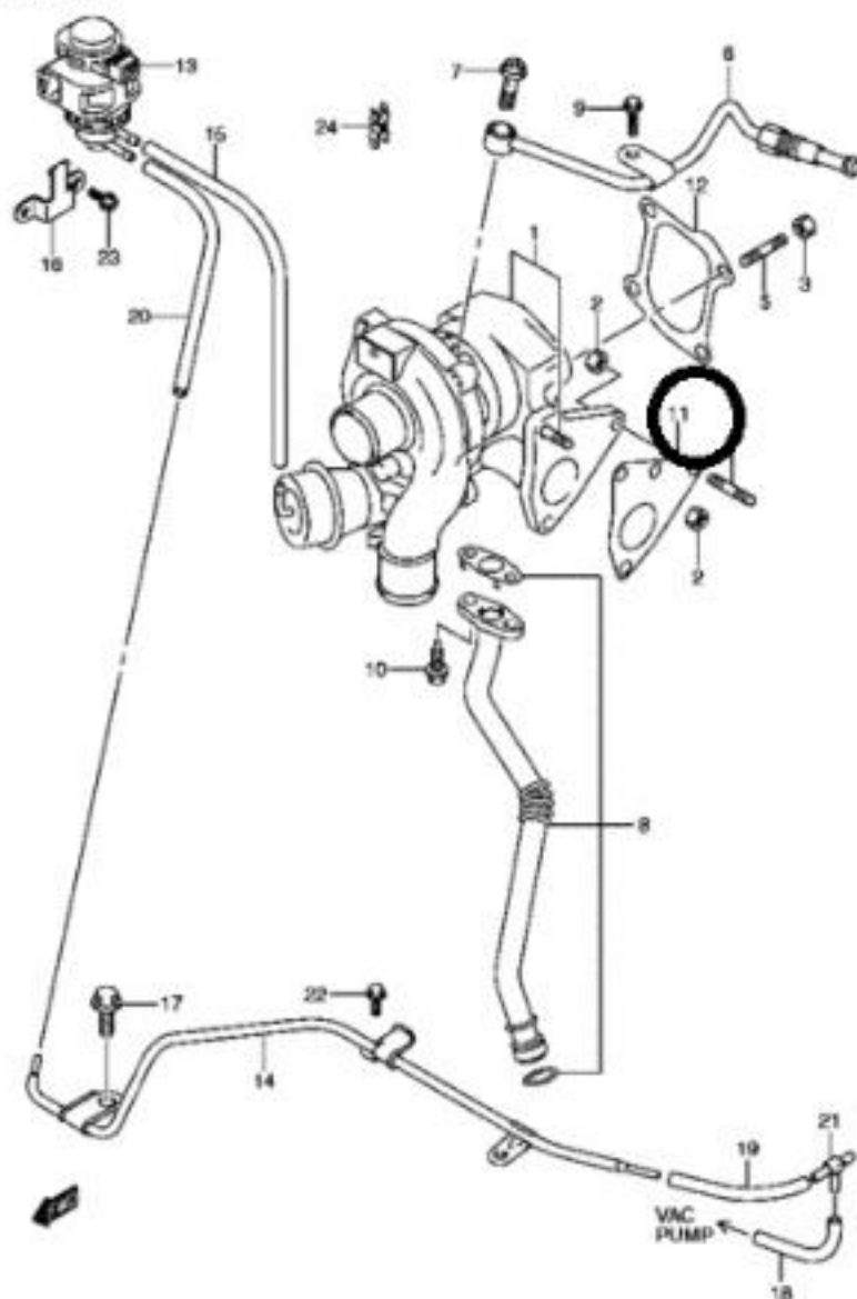
SN413V-5 E22_032A TURBO CHARGER (SN415VD-2)
