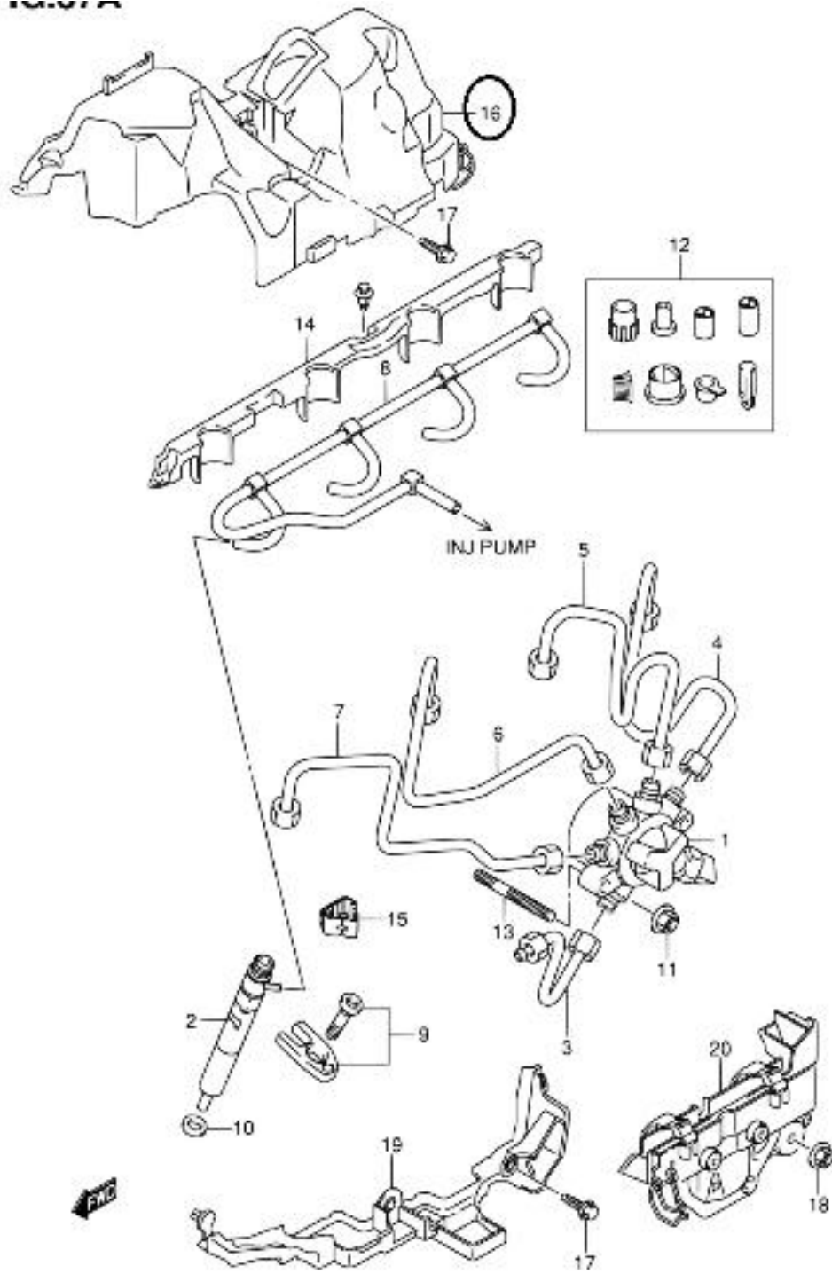
SN413V-5 E22 037A FUEL INJECTOR (SN415VD.2)
