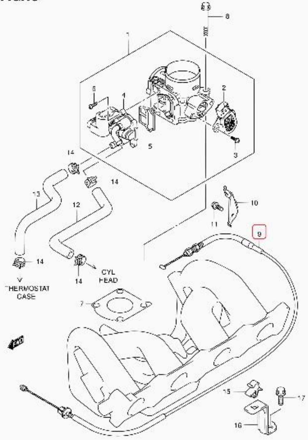
SN413V-2 E22 018 THROTTLE BODY (SN413V)
