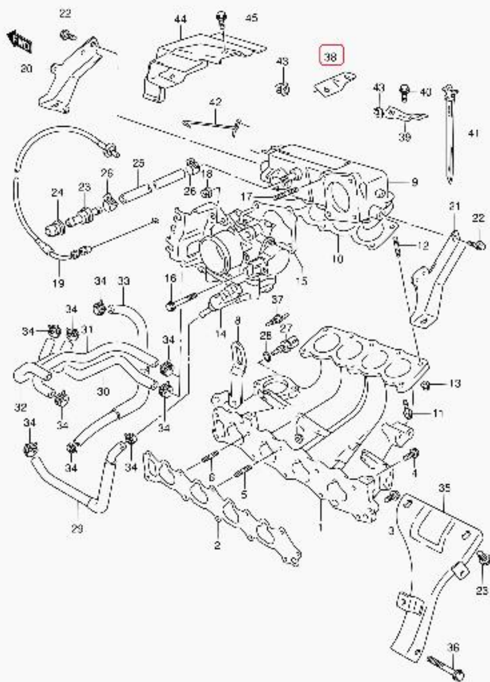
SE416 3DR E01 032 INTAKE MANIFOLD/THROTTLE BODY (13)
