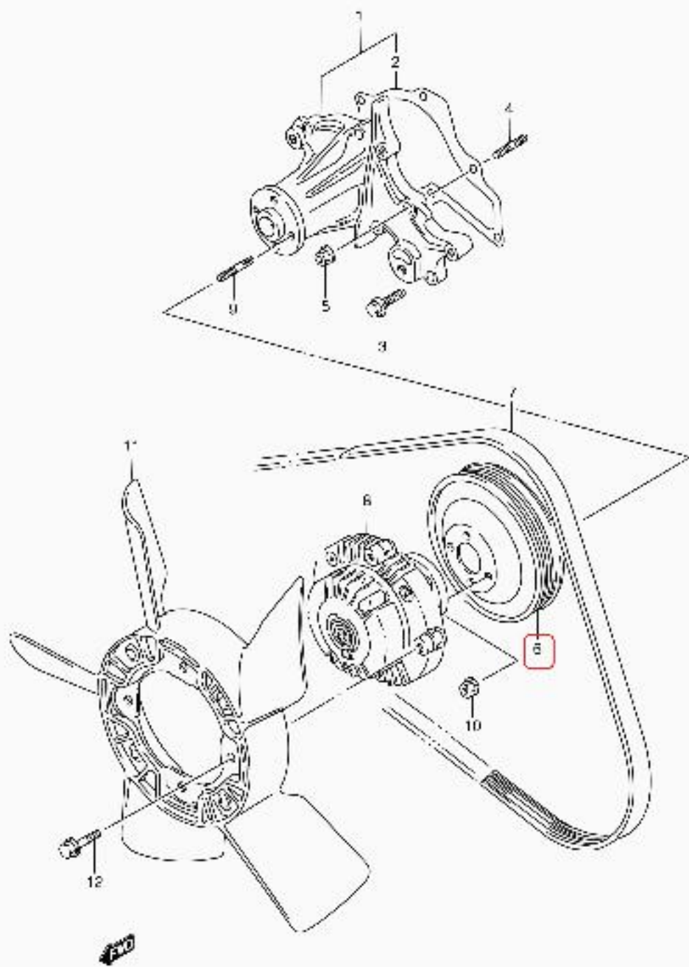
SQ416L/420L E30_036 WATER PUMP:SQ416L
