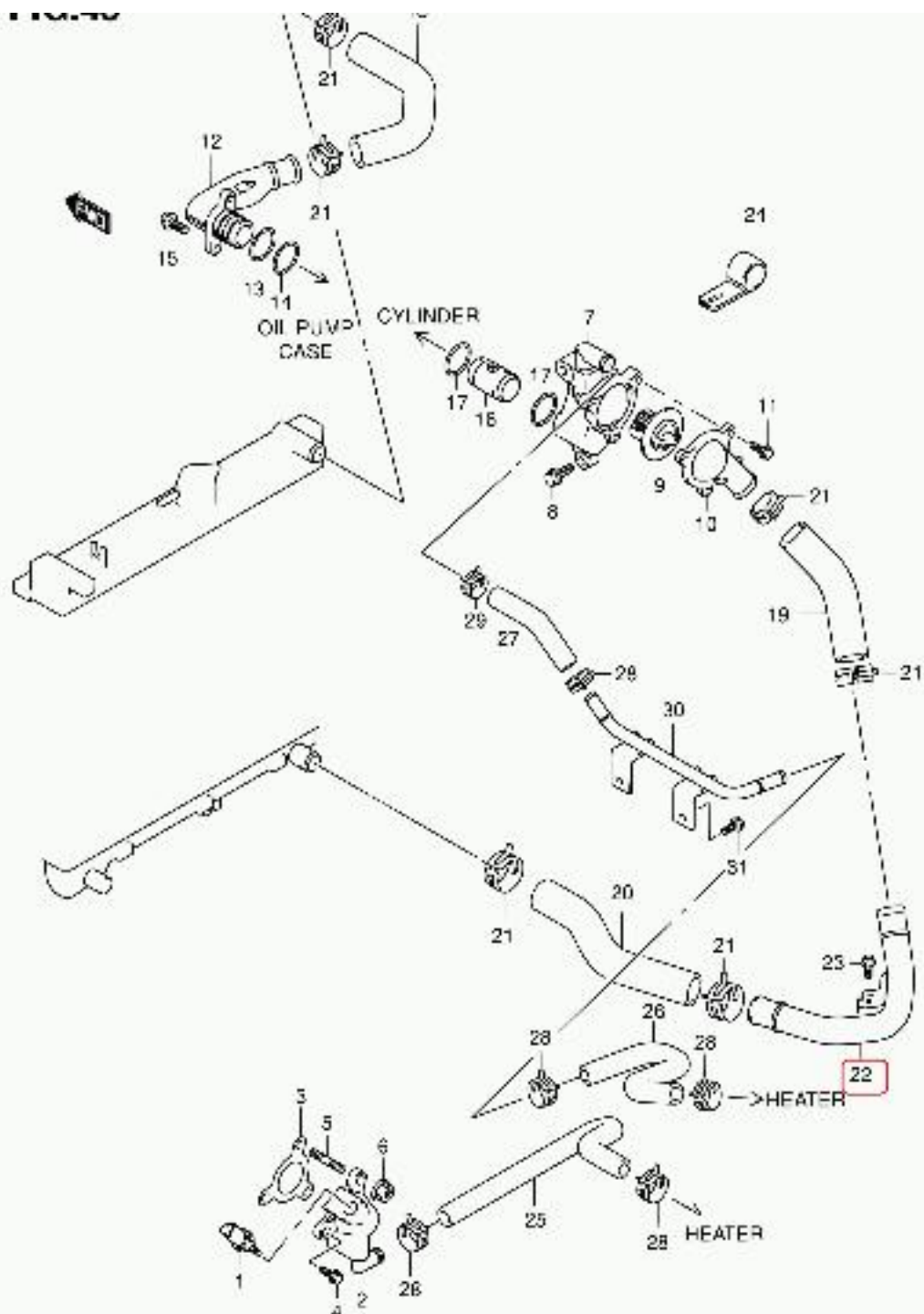
SN413V-5 E22 045 WATER HOSE (SN413V)
