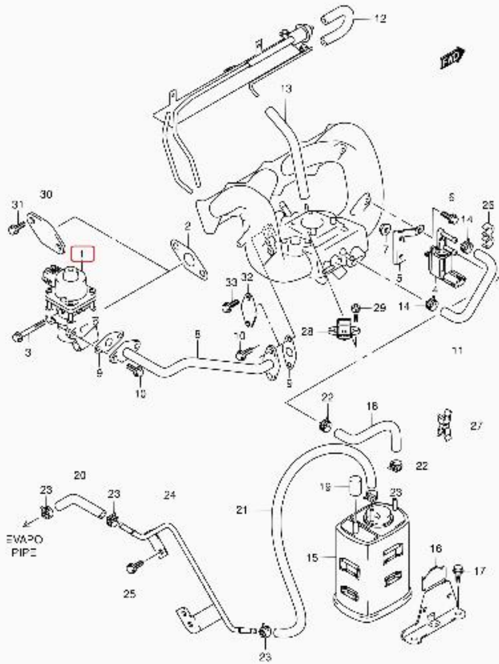
SM413V-5 E22 047 EMISSION CONTROL (SM413V)
