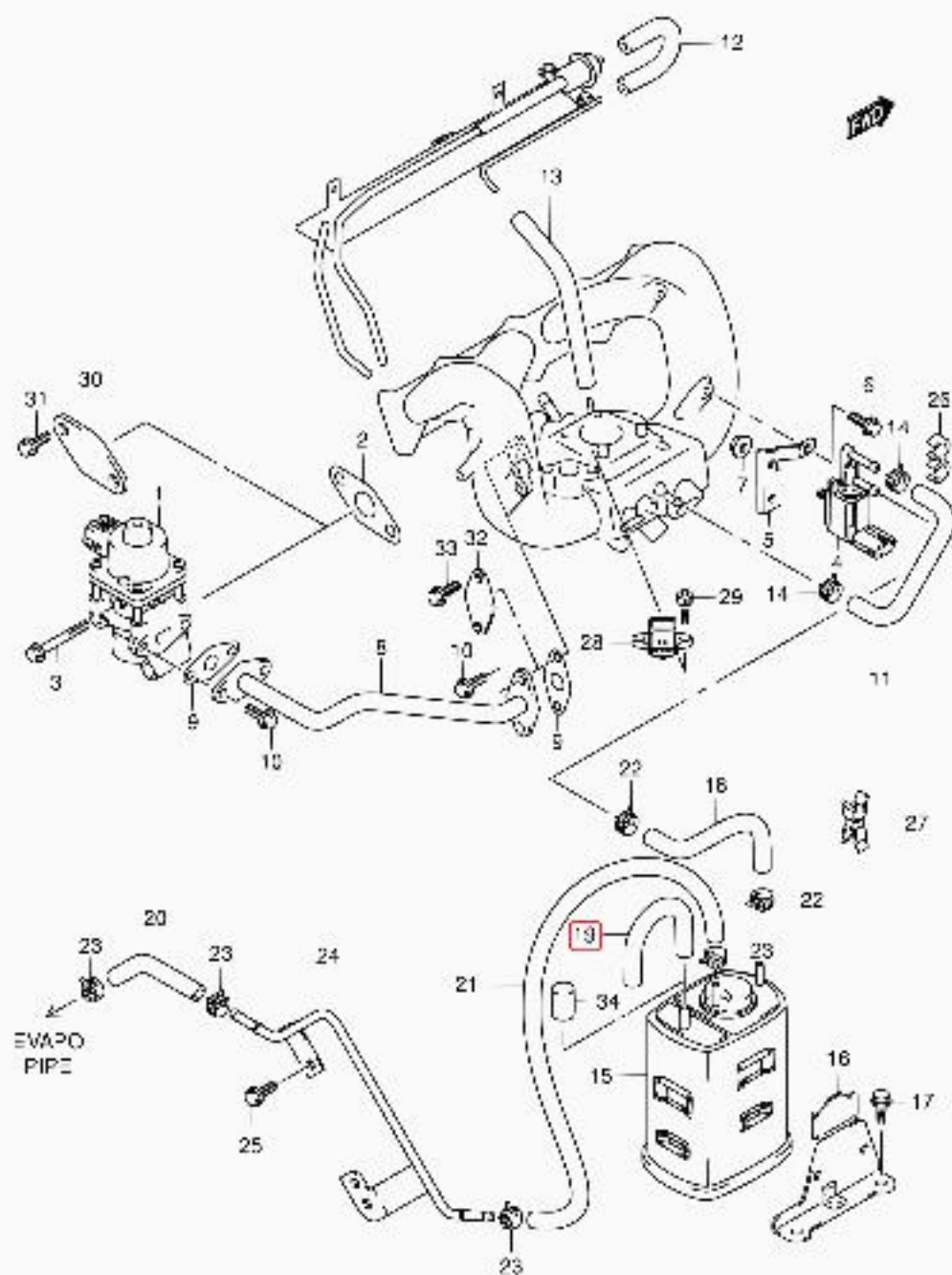
SA413V-2 E22 042 EMISSION CONTROL (SA413V)
