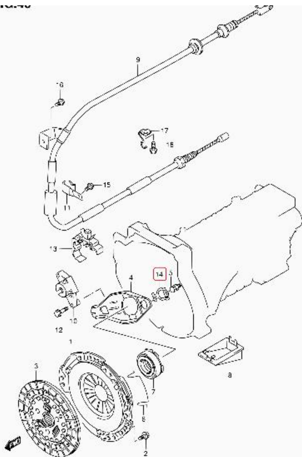
SN413V-2 E22 048 MT CLUTCH (MT:L43:SN413V)
