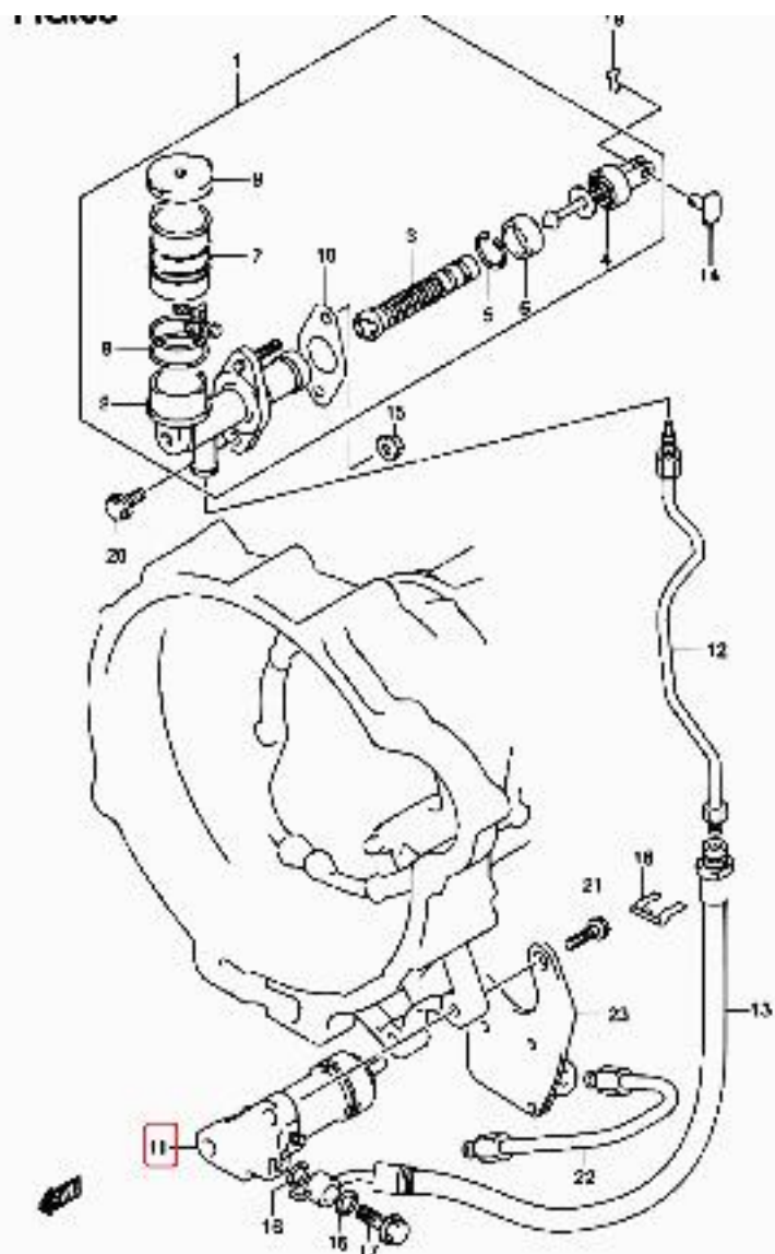
SQ420W-3 E22_063 MT CLUTCH MASTER CYLINDER (MT:SQ420W)
