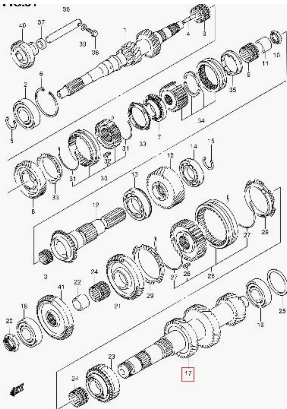
SK413V-2 E22 051 MT TRANSMISSION (MT:SK415VD)
