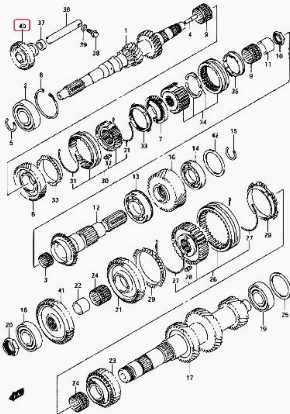
JB627W E33_025 MT TRANSMISSION (MT)
