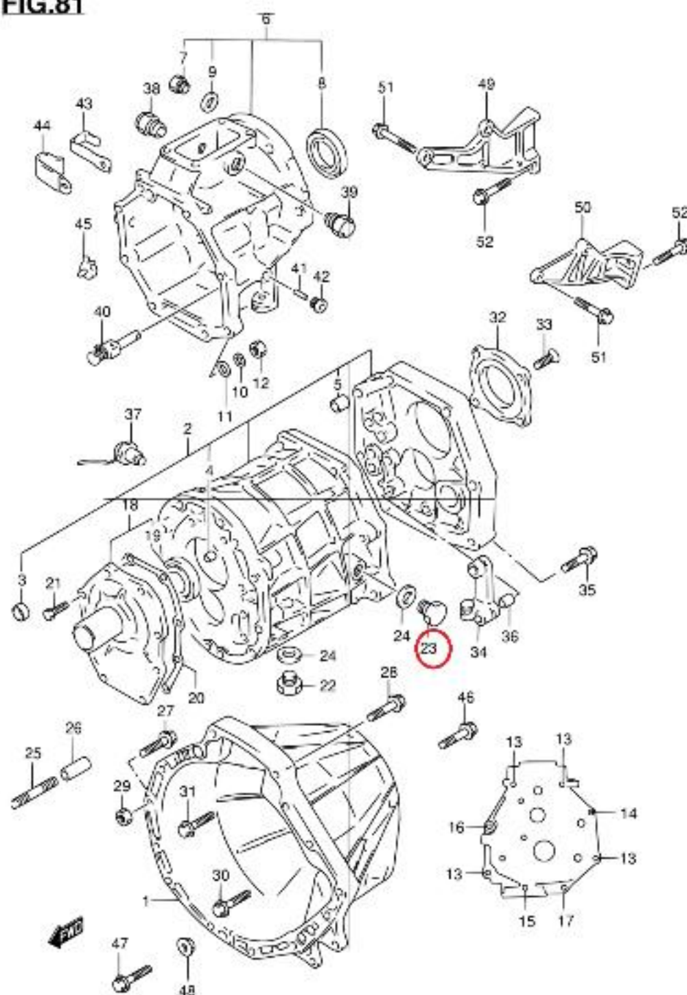
SQ420W E22_081 MT TRANSMISSION CASE (420WD,625W)
