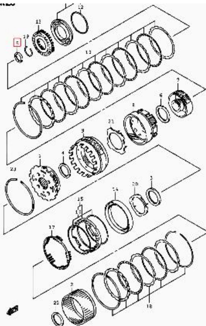
GA413 MT K55_025 MT PLANETARY GEAR
