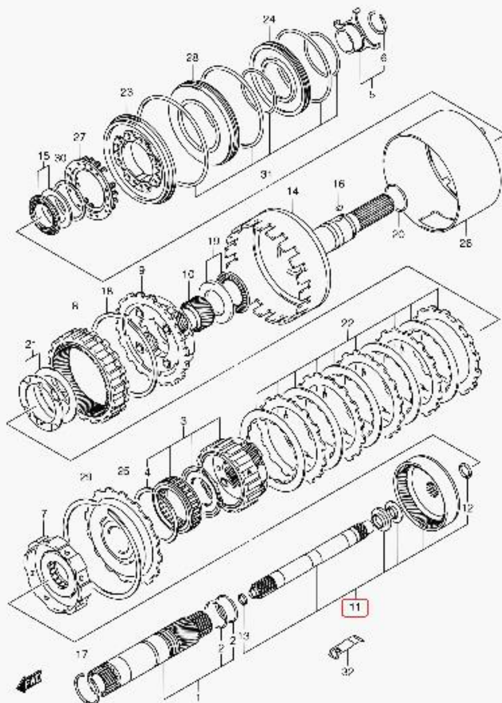
JB416X-4 E22_083 AT PLANETARY GEAR
