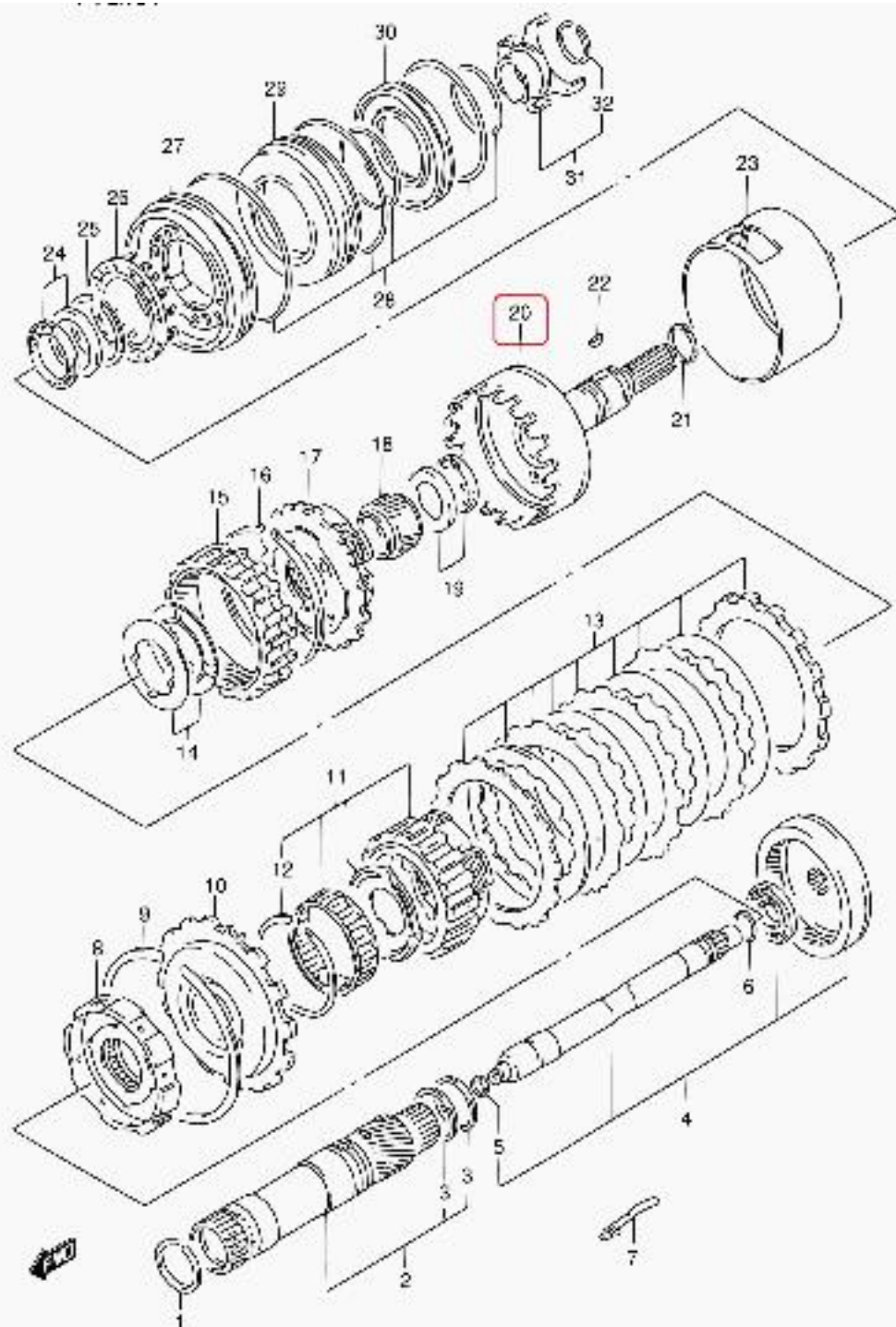
SQ420Q E22 C57 AT PLANETARY GEAR(AT)
