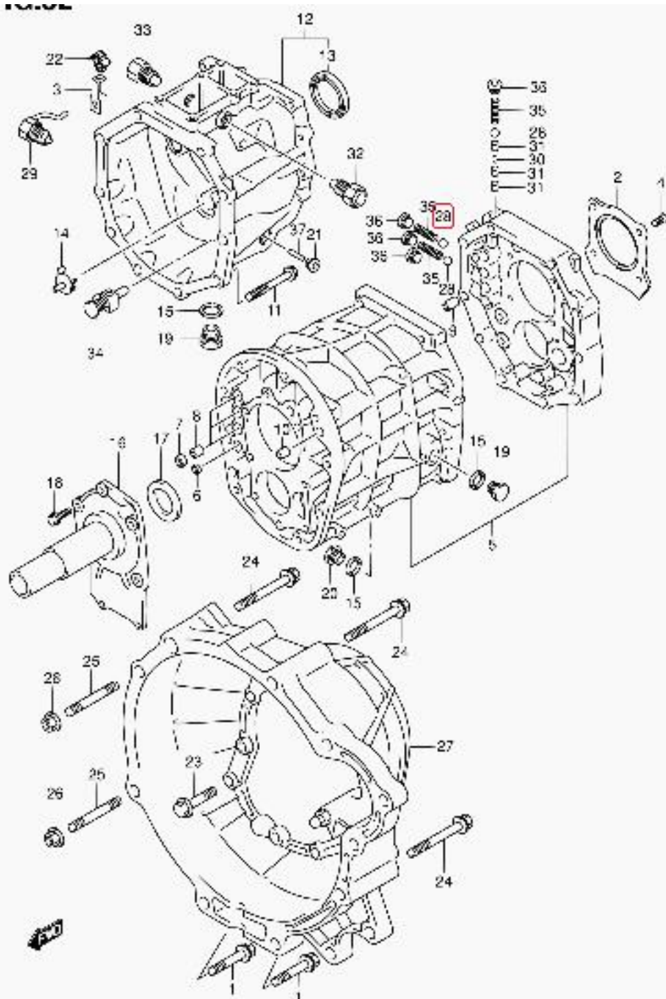
SQ416V-3 E22 082 MT TRANSMISSION CASE (MT:SQ420WD)
