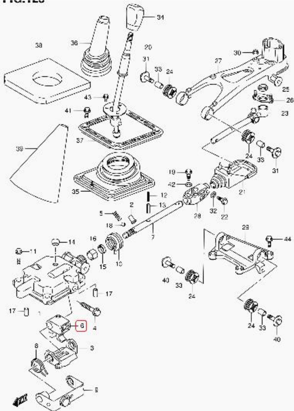
JB420W-4 E22 125 GEAR SHIFT CONTROL (1)
