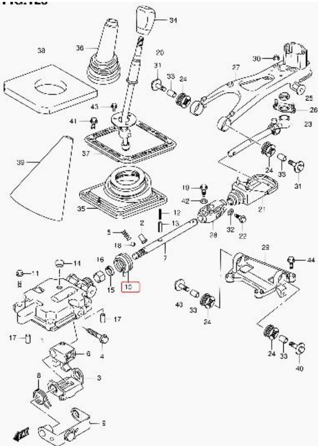
JB420W-4 E22 125 GEAR SHIFT CONTROL (1)
