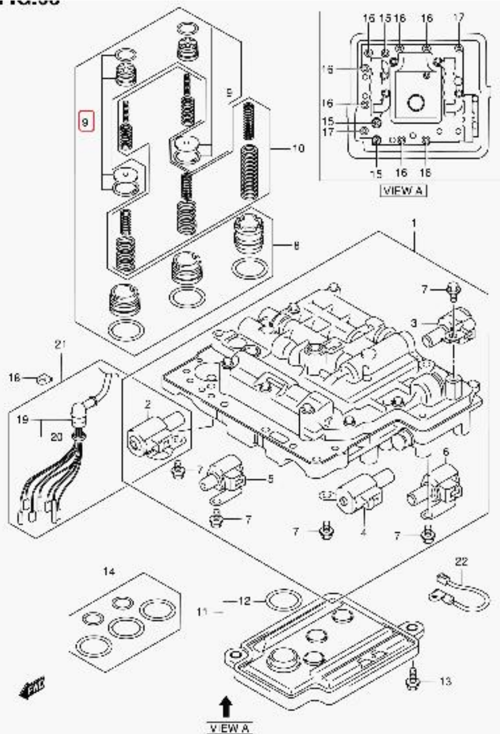
SA413V-2 E22 063 AT VALVE BODY (AT)
