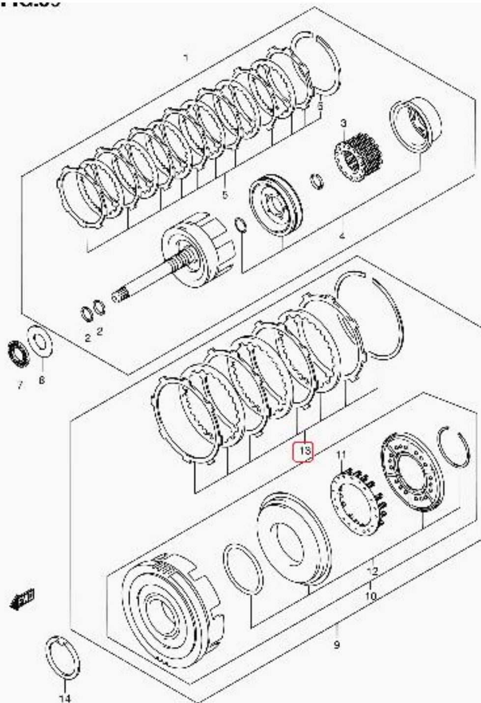
SA413V-2 E22 058 AT INPUT SHAFT (AT)
