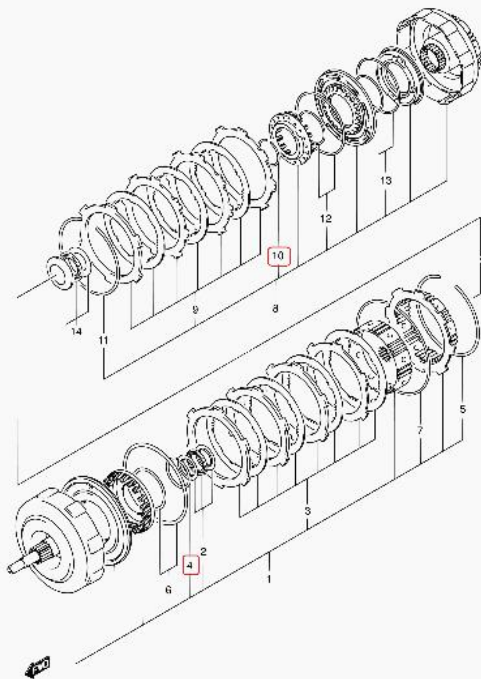
JB420W-4 E22 10E AT FORWARD CLUTCH (JB420W, JB424W)
