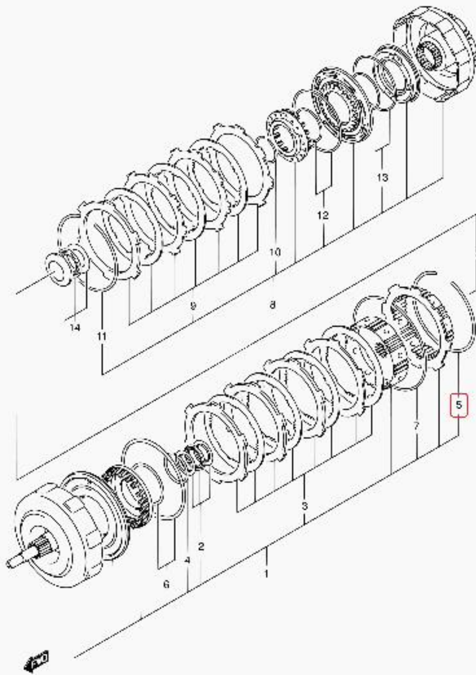
JB416X-4 E22 084 AT FORWARD CLUTCH
