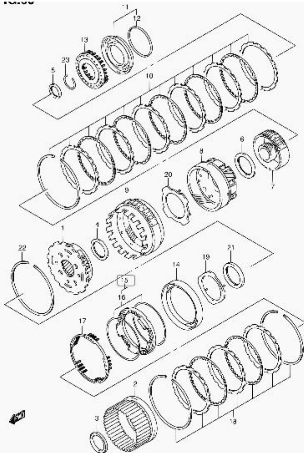
SA413V-2 E22 060 AT PLANETARY GEAR (AT)
