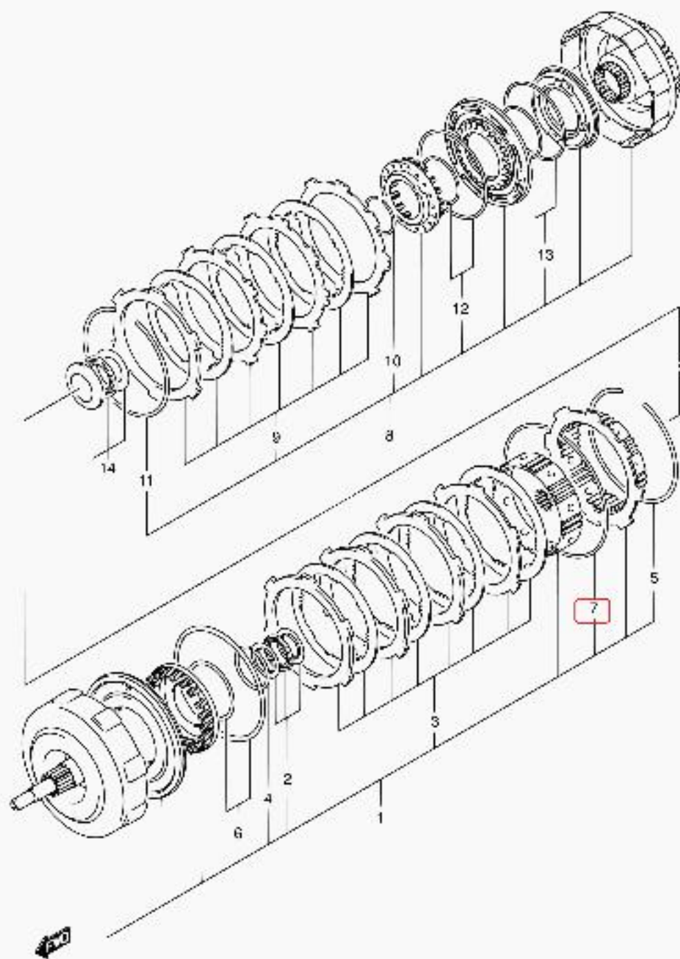
JB420W-4 E22 10E AT FORWARD CLUTCH (JB420W,JB424W)
