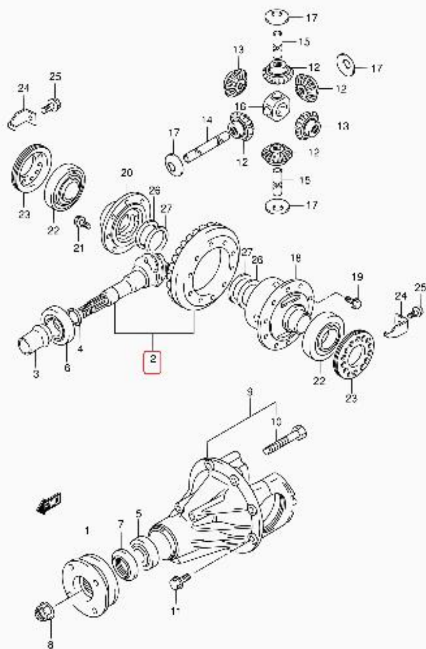
SA413V-2 E22 075 REAR DIFF GEAR
