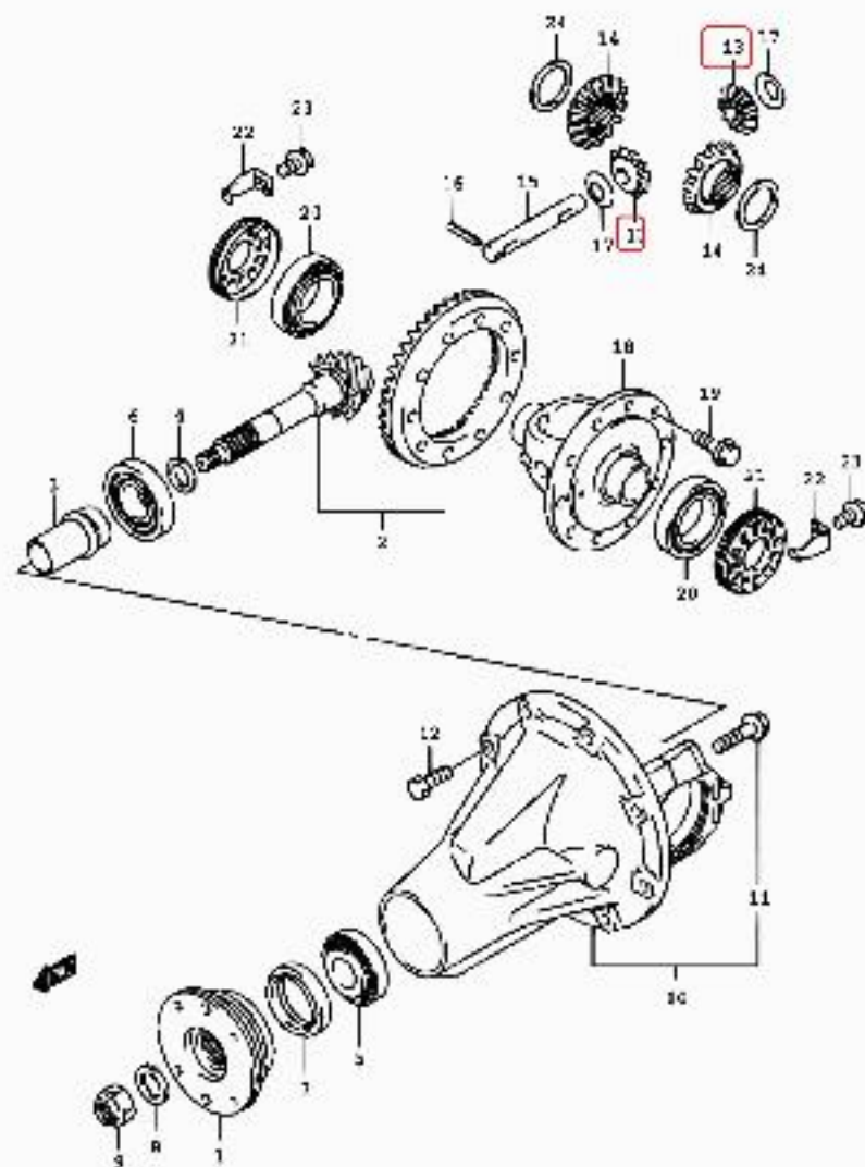
GA413 AT E35_034 REAR DIFF GEAR
