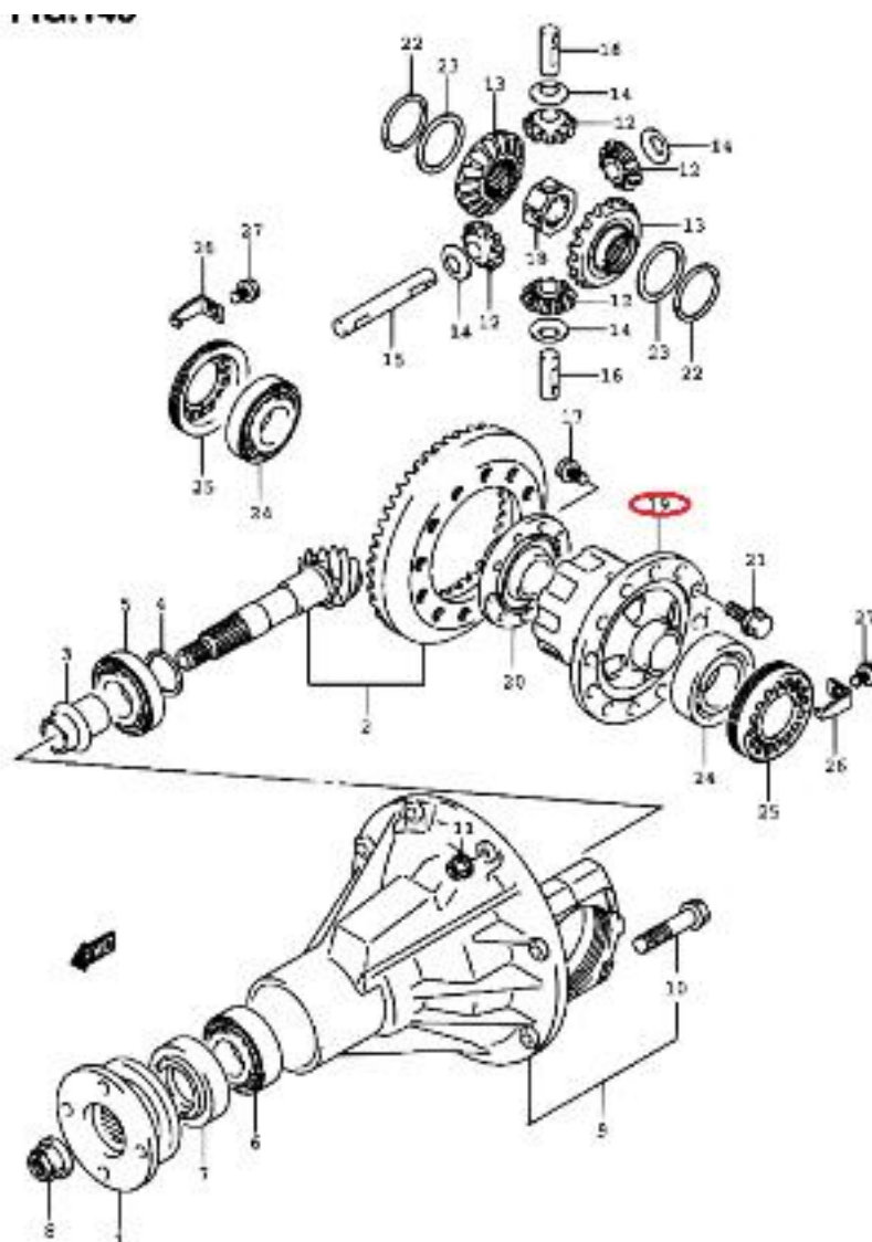
SQ420W-2 B22_145 REAR DIFF GEAR (SQ420W, SQ420WD, RP, SQ625W)
