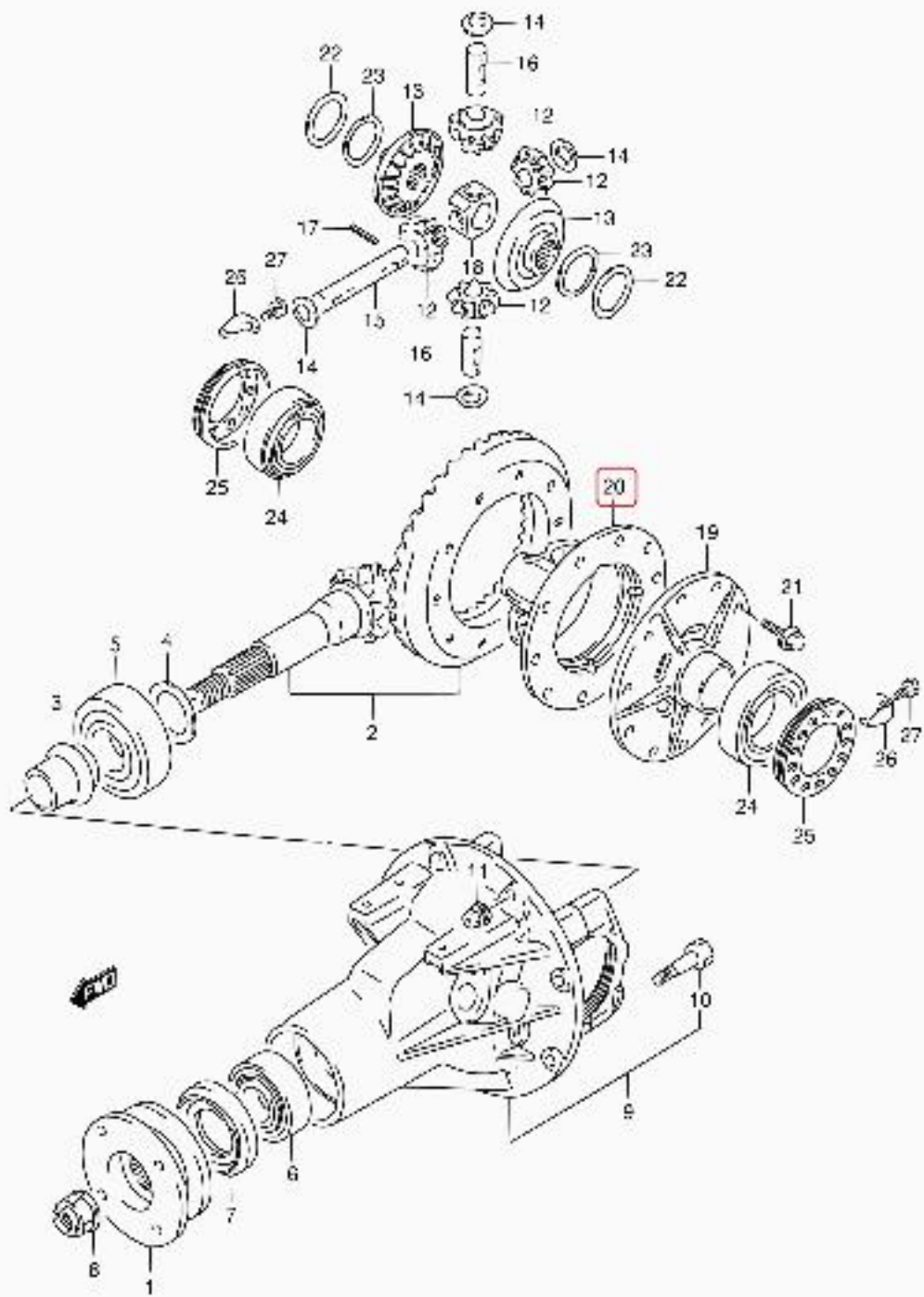
SQ420Q E22_069 REAR DIFF. GEAR(AT)
