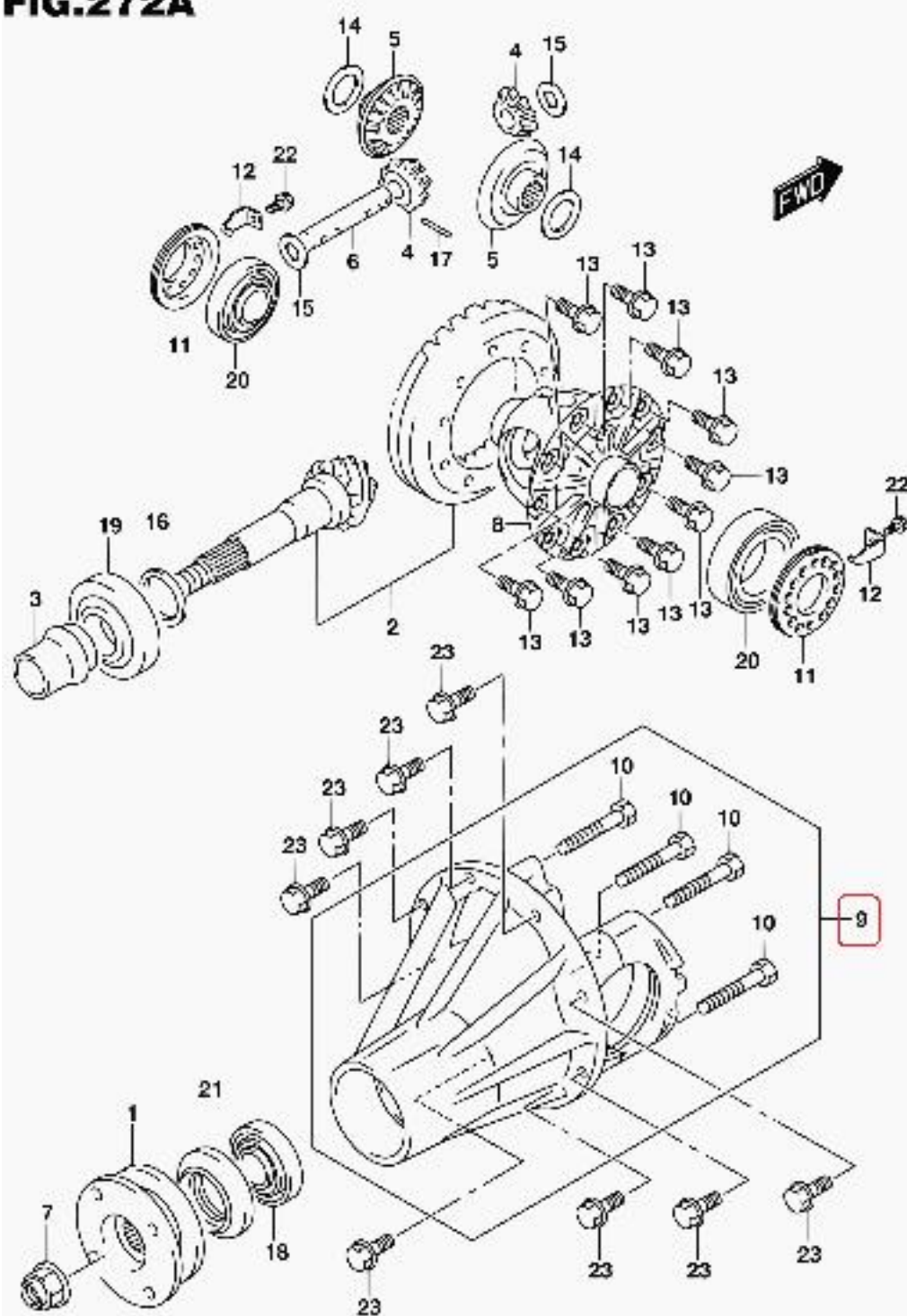
AEG415 E24 272A FRONT DIFF GEAR
