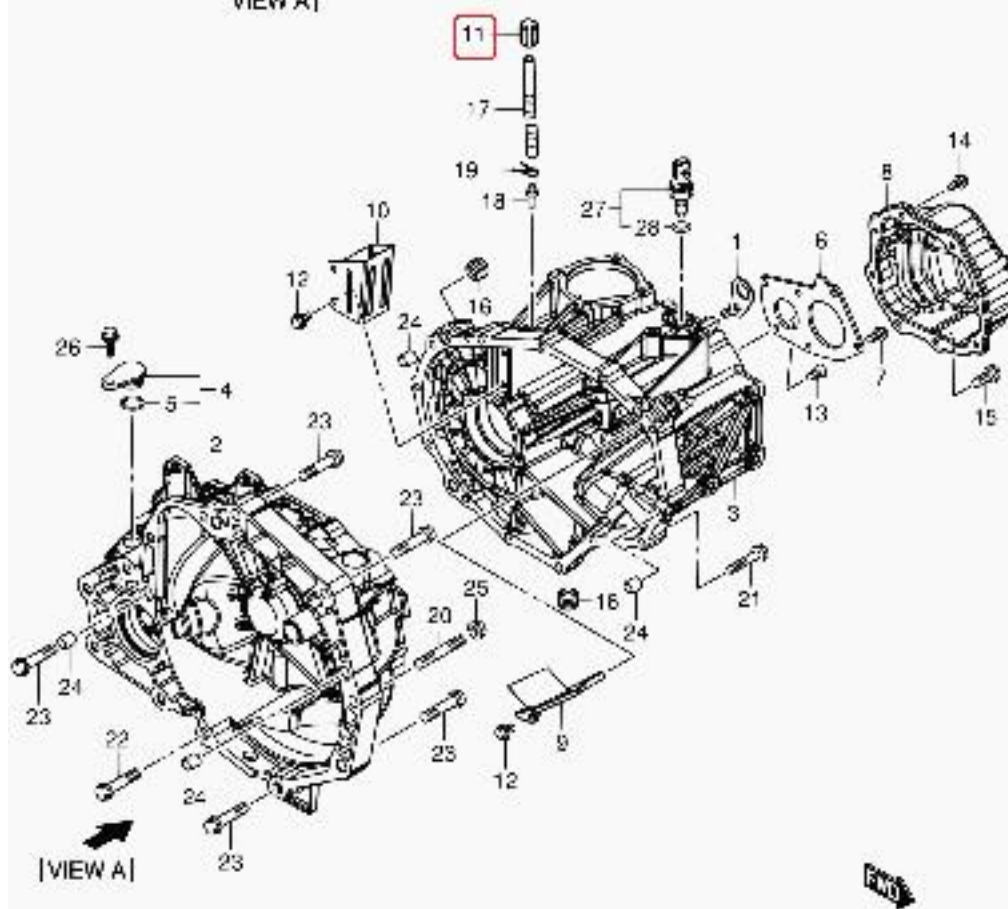
VIEW A
